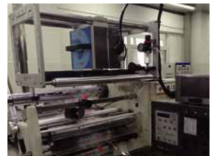
D05S installed on FFS Machine
